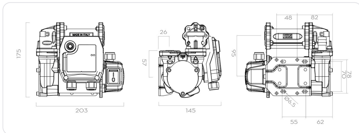
PIUSI 3000 Supreme vertical ports, dimensions in mm
