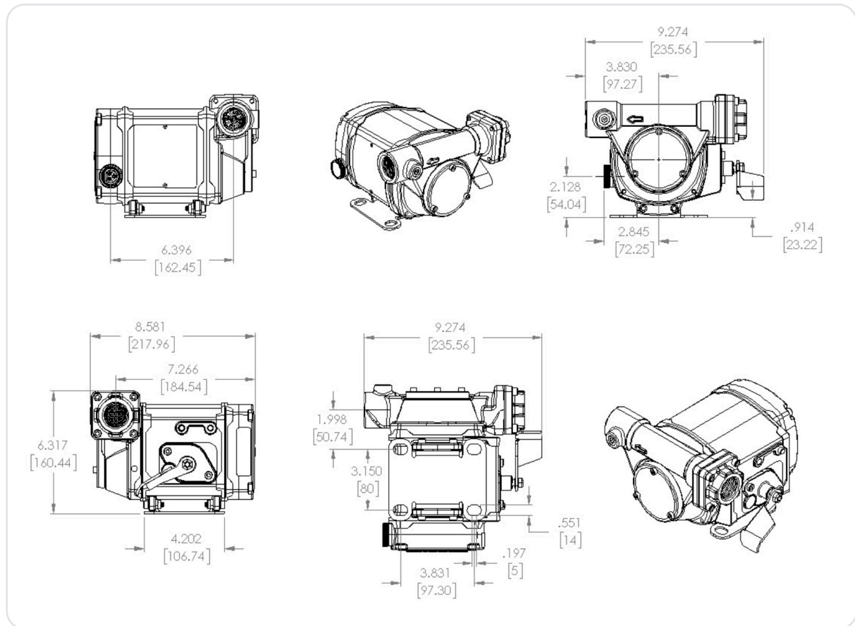
Foot mount model dimensions, inches [mm]
