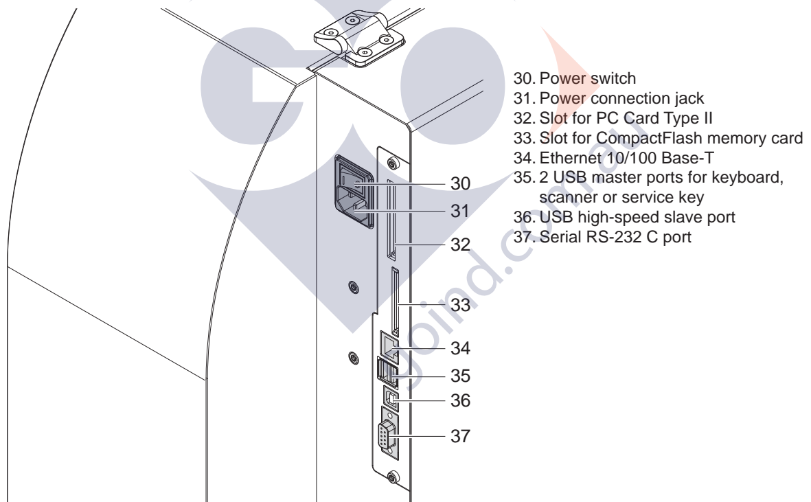
Fig. 4 Connections
