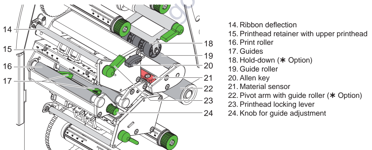
Fig. 2 Print mechanics - upper print unit
