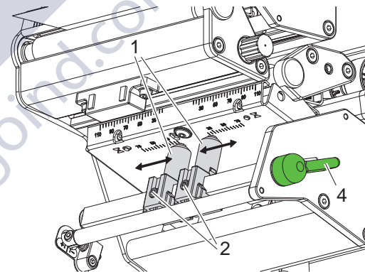
Fig. 16 Setting the lower head locking system
