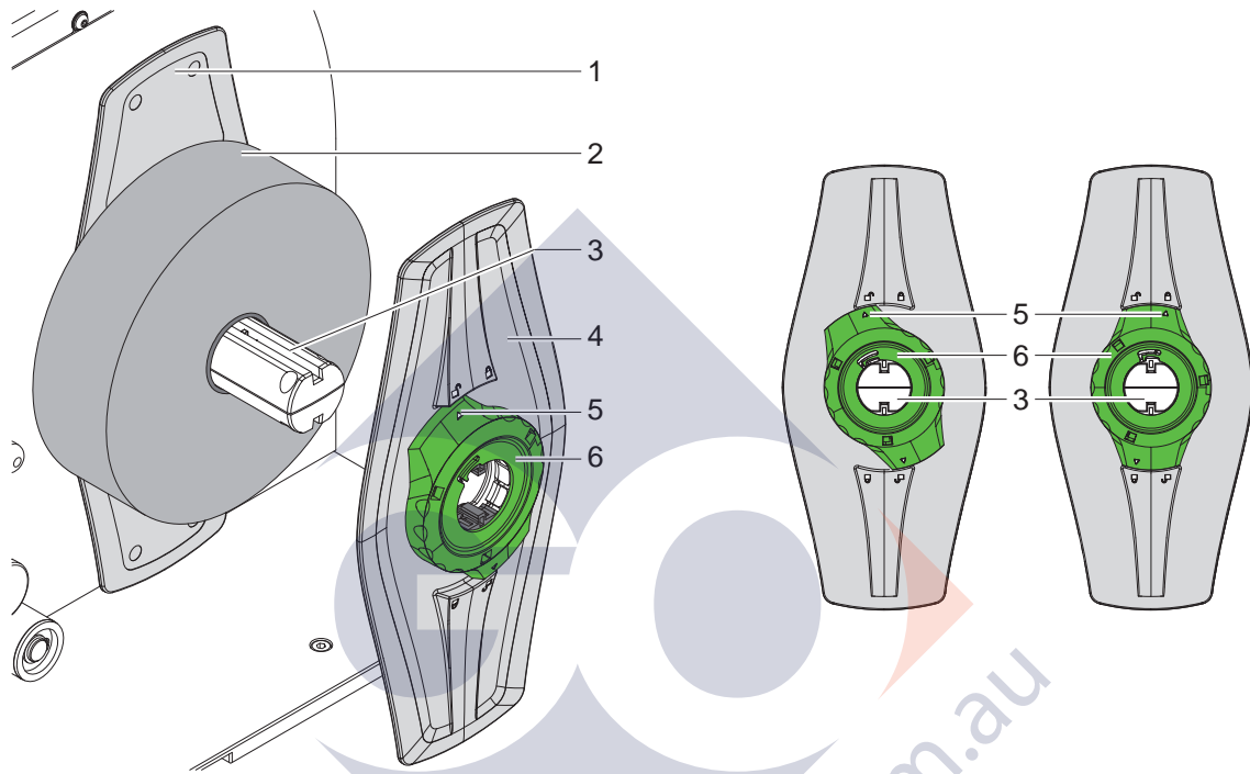
Fig. 6 Loading media from roll
