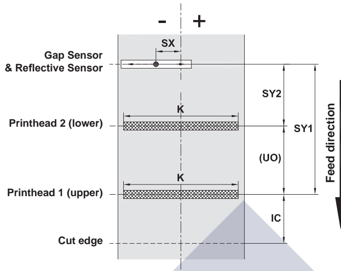
Fig. 18 Device dimensions
