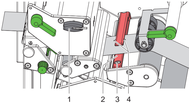
Fig. 10 Setting the material sensor
