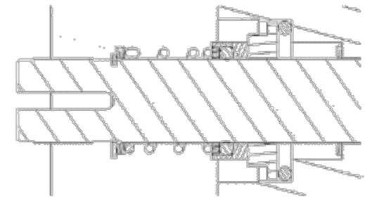
Shaft Seal Assembly – KIT700SL
