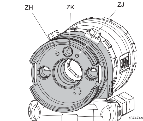
FIG. 3 Fluid Housing Passages
