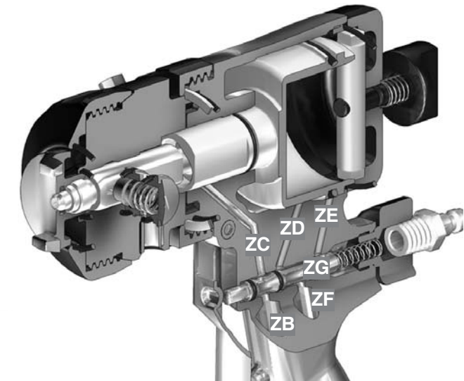
FIG. 2 Gun Handle Passages
