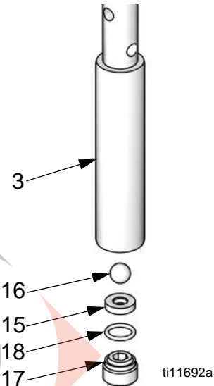
FIG. 5. Replace piston ball and seat.
