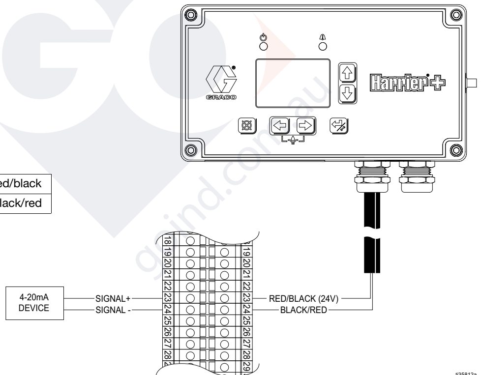
FIG. 11: Non-Powered Device, use terminals 23 and 24
