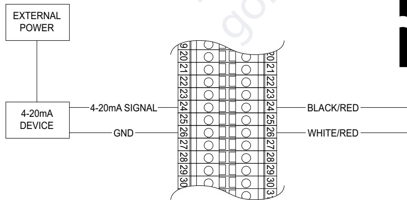
FIG. 9: Powered Device, use terminals 24 and 26
