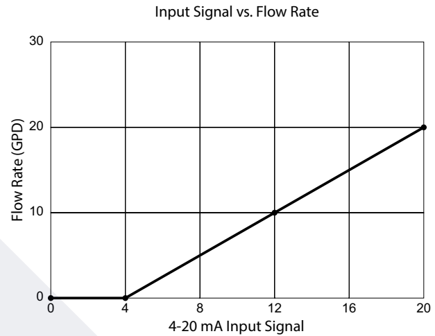
FIG. 51: Full Range Setup
