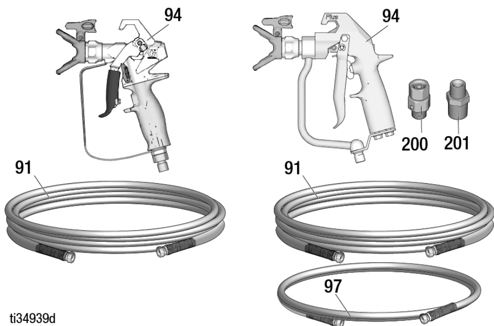
Figure 14-10: Spray Gun and Hose Parts Diagram
