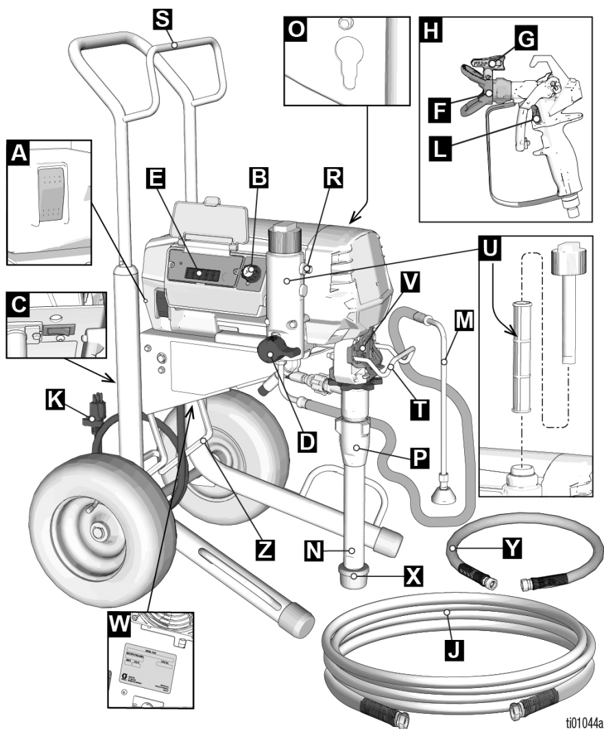
Figure 6-1: Components for Standard Models
