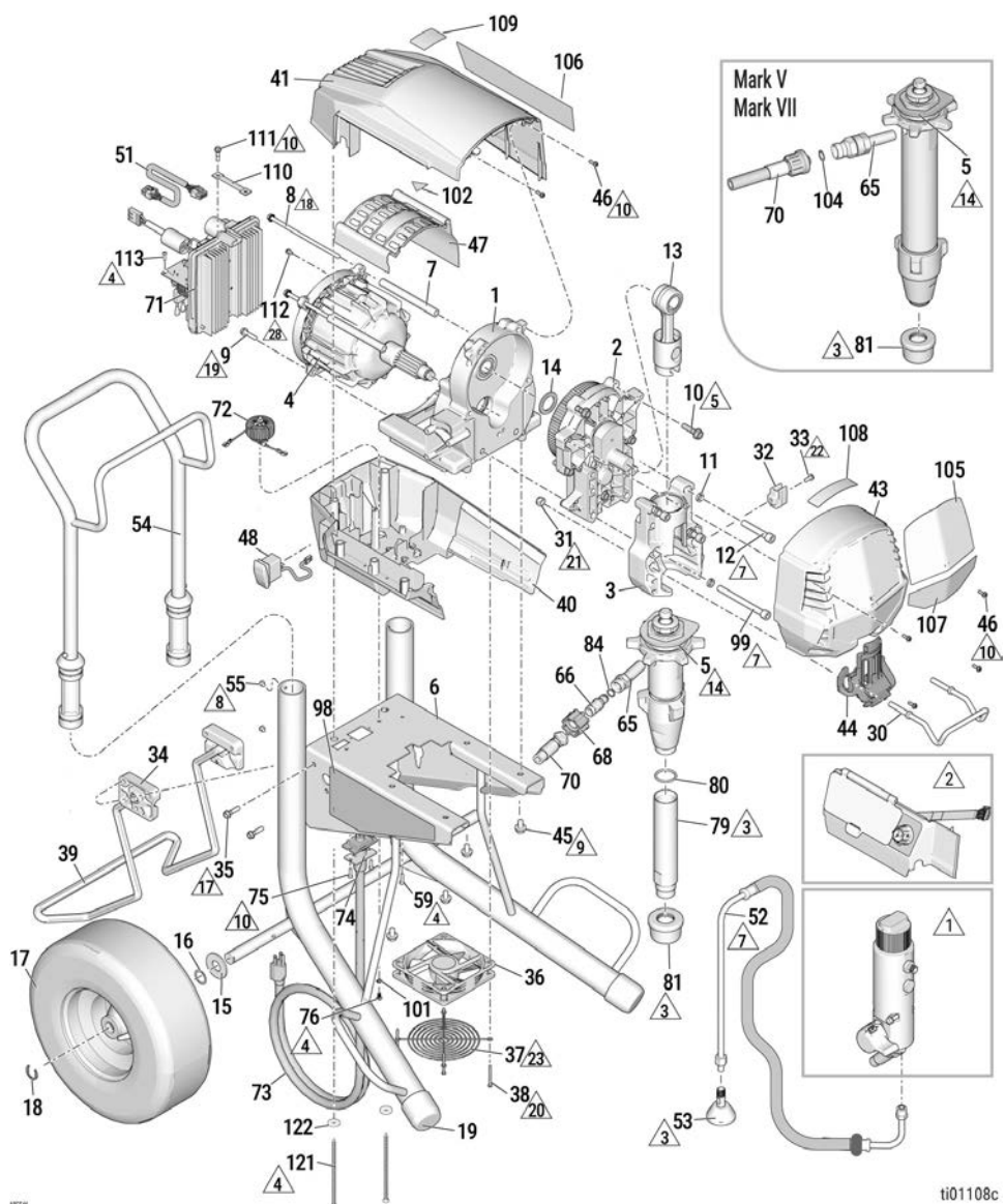
Figure 14-3: 1095 XT, Mark V, Mark VII Standard Hi-Boy Parts Diagram
