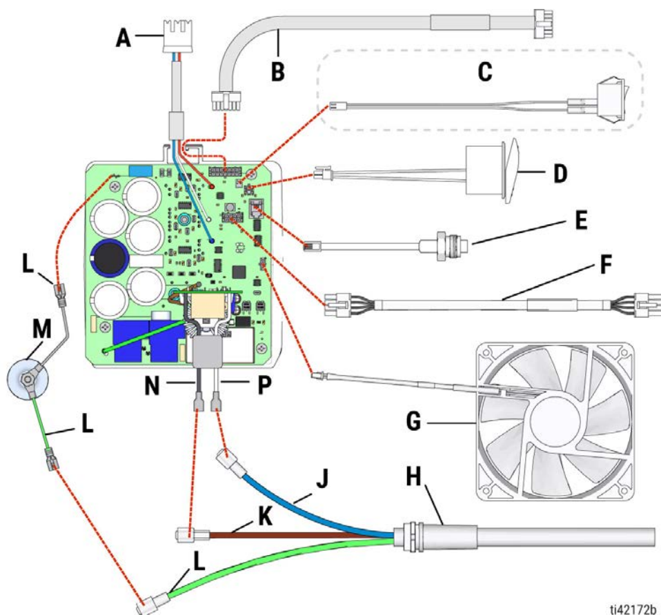
Figure 16-2: Wiring Diagram for 110 V UK
