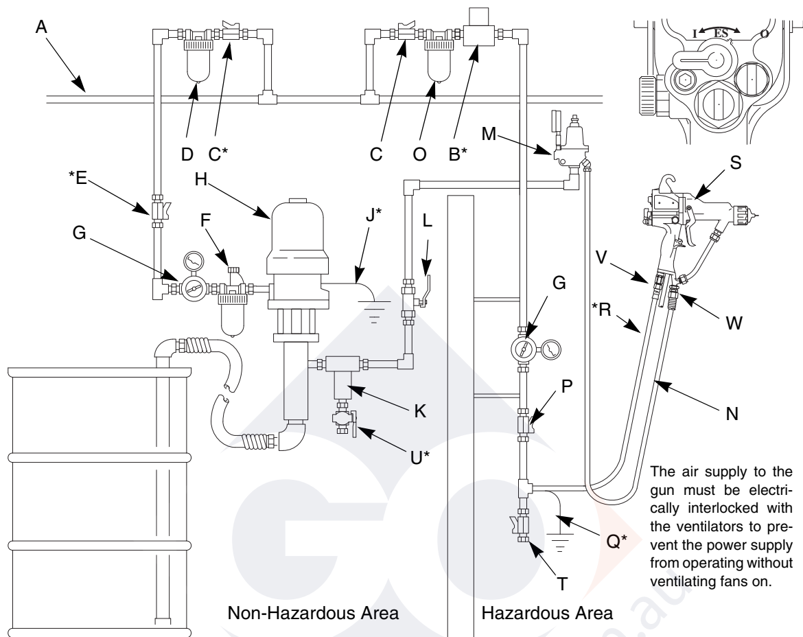
Fig. 2. Typical Installation
