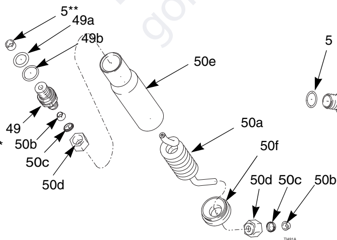
Fluid Tube: Model 244576
