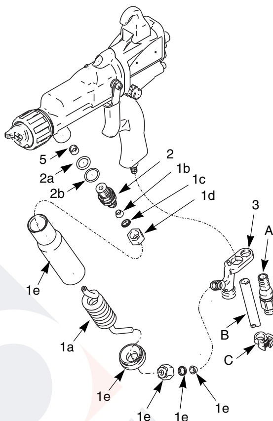
FIG. 3: 244919 Conversion Kit
