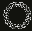
RANDOM ORBITAL
